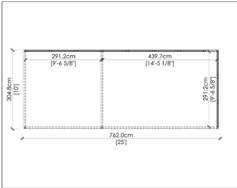
1 TOP VIEW
