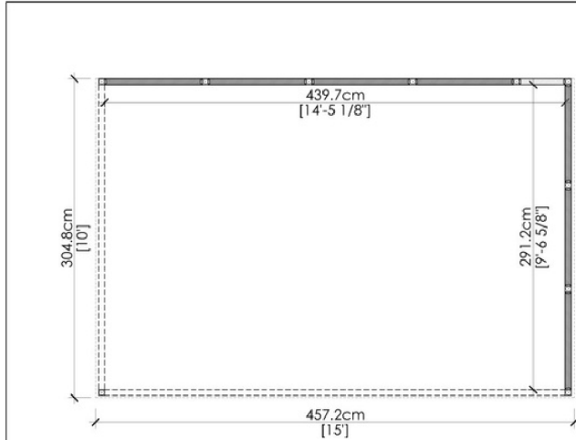
1 TOP VIEW
