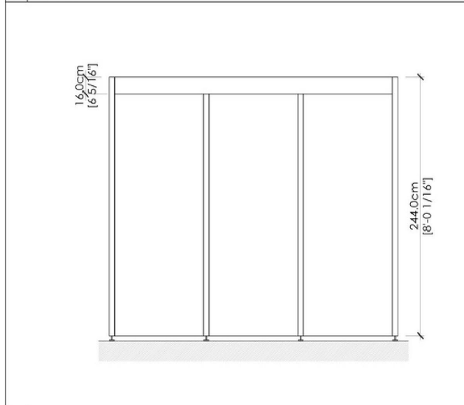
2 FRONT VIEW
