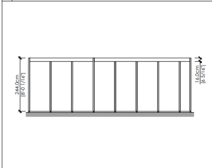
2 FRONT VIEW
