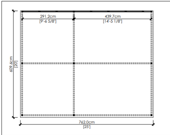
1 TOP VIEW
