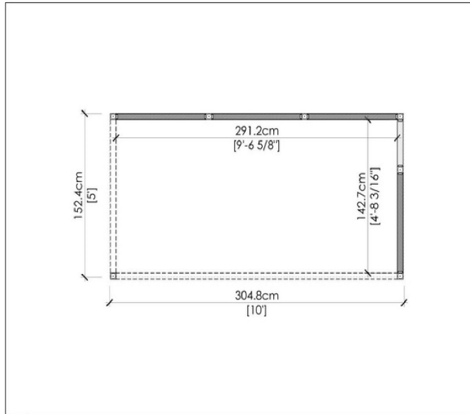
1 TOP VIEW
