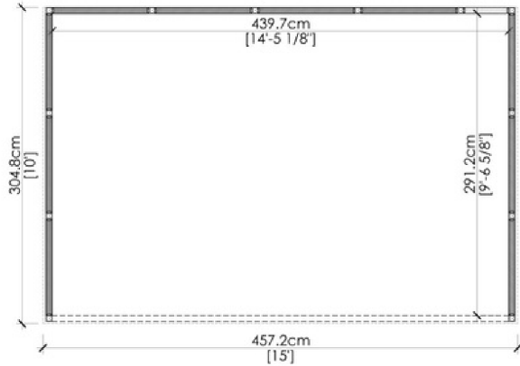
1 TOP VIEW
